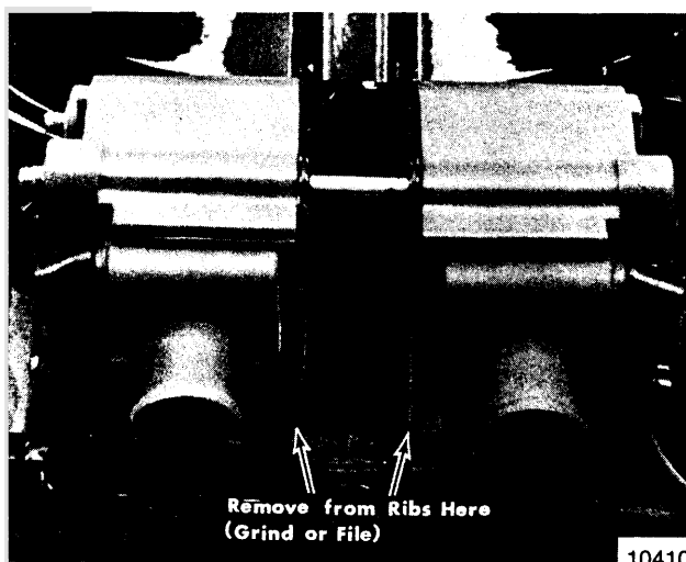
Figure 1. Starter Housing in Contact with Cylinder Block
