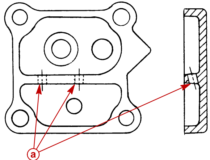
a - Cross Flow Holes Figure 1.
