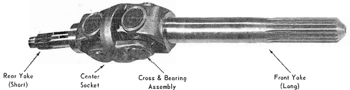
Figure 5. Universal Joint Assembly Components
