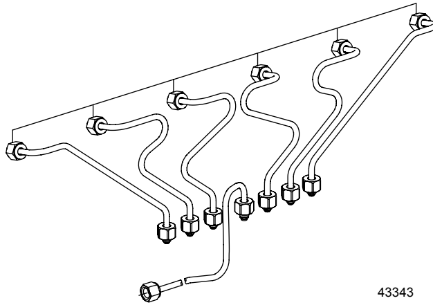
High-pressure fuel line kit
