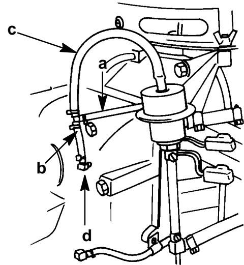
a - Tigon Hose Between Throttle Position Indicator and T-fitting (Remove) b - T-fitting and Short Tigon Hose (Remove) c - Fuel Pressure Regulator Tigon Hose d - Air Inlet Plenum Fitting
