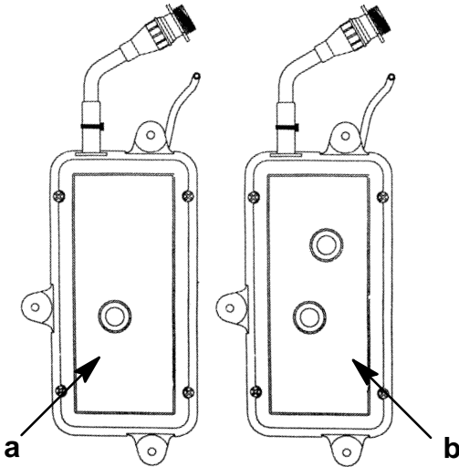
a - Analog 11350 ECU b - Digital 11350 ECU
