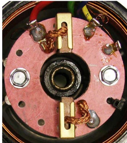
Correctly soldered terminals
