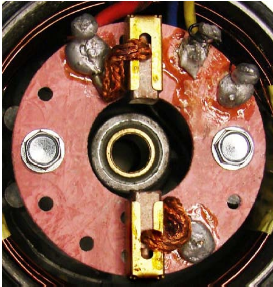
Incorrectly soldered terminals
